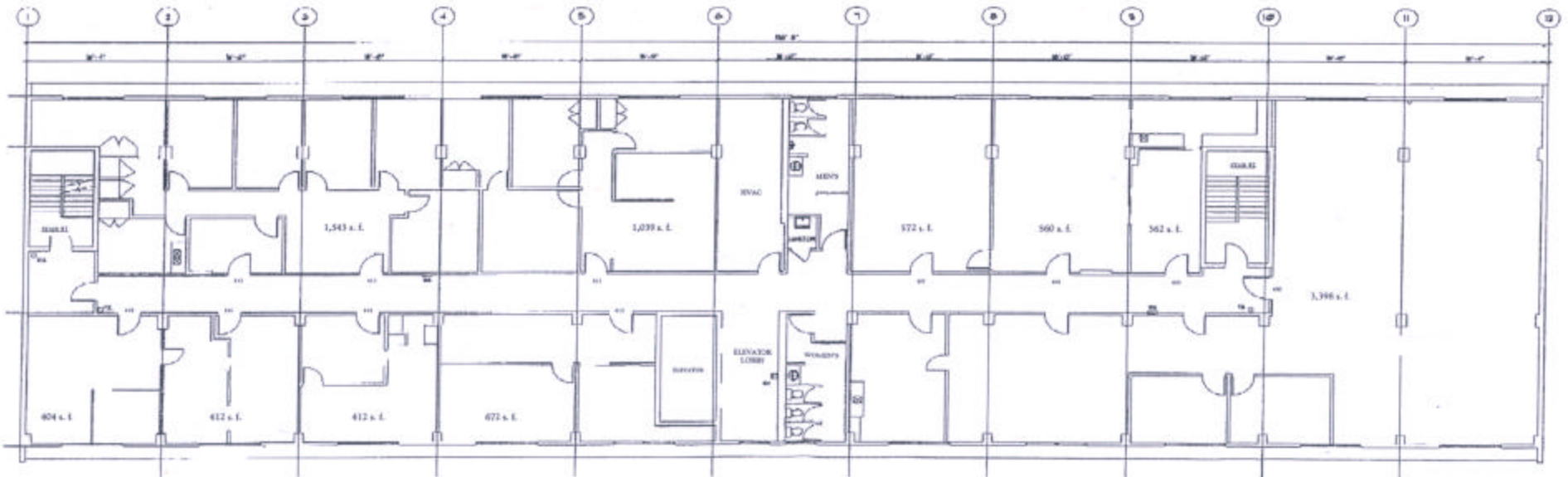
FOURTH FLOOR PLAN (AS-BUILT)
