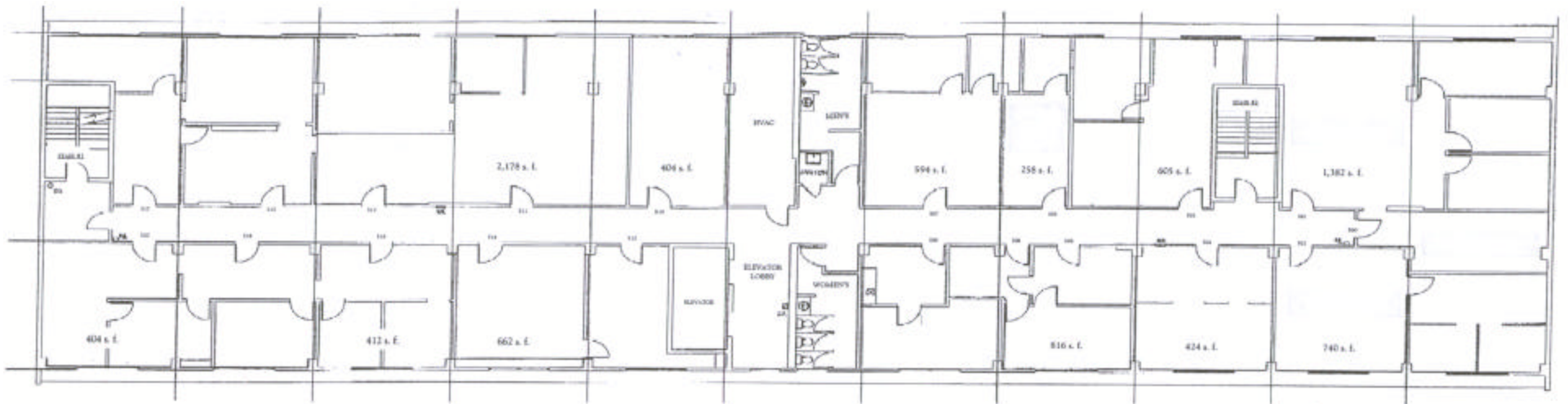
FIFTH FLOOR PLAN (AS-BUILT)
